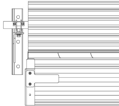
FIGURE 23: HEADSTOPS
