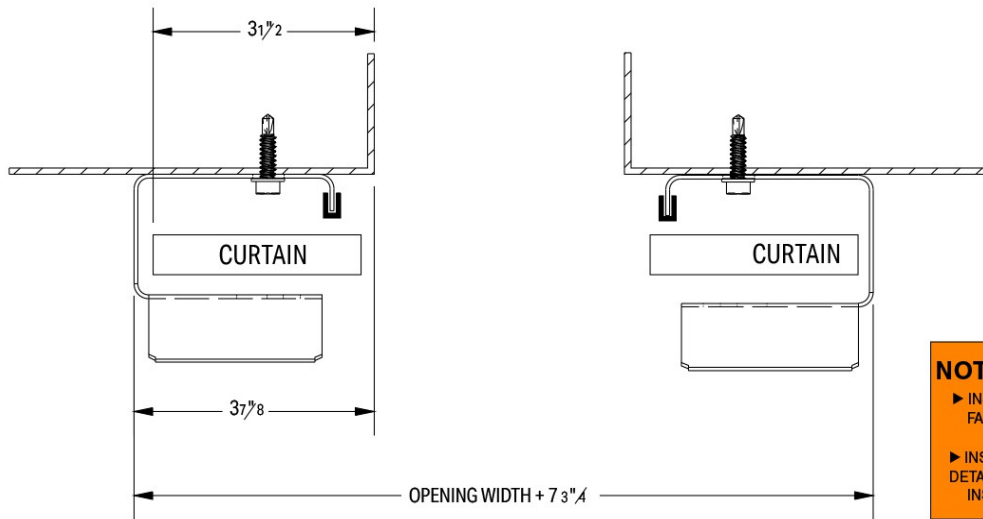
FIGURE 18: STEEL JAMBS
