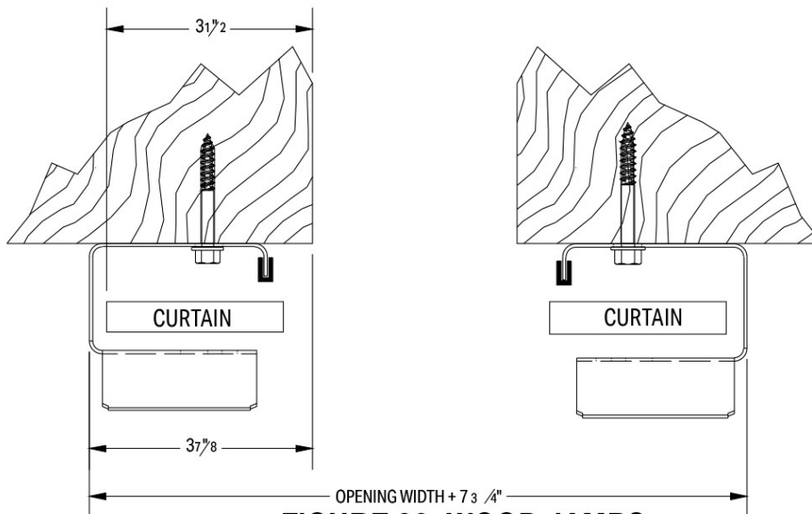
FIGURE 20: WOOD JAMBS
