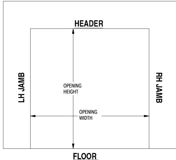
FIGURE 4: WALL OPENING
