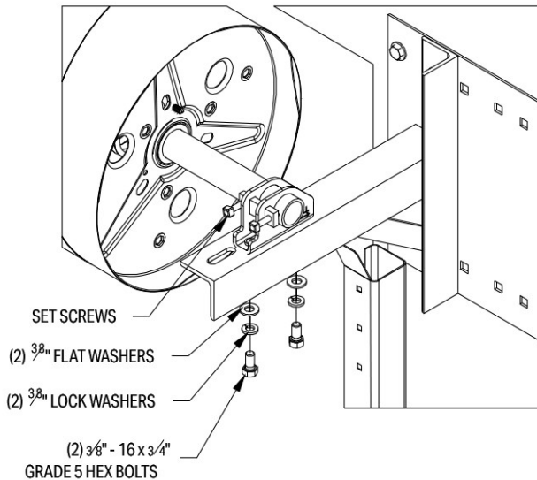
FIGURE 14: SECURING SADDLE
