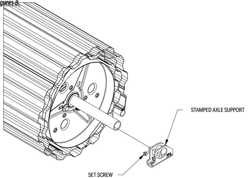
FIGURE 8: SECURING THE STAMPED AXLE SUPPORT
