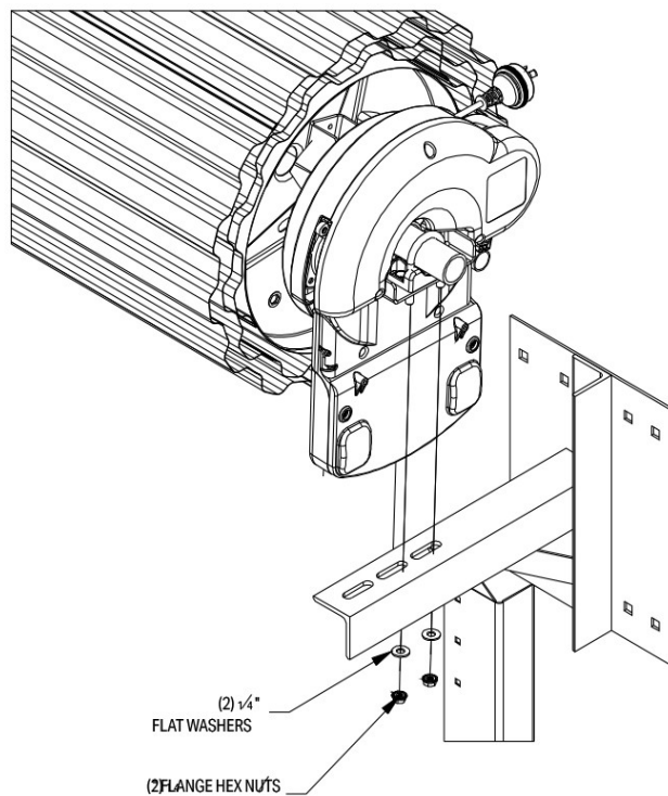
FIGURE 17: ATA OPERATOR END
