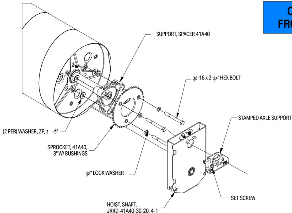
FIGURE 9: CHAIN HOIST 4:1
