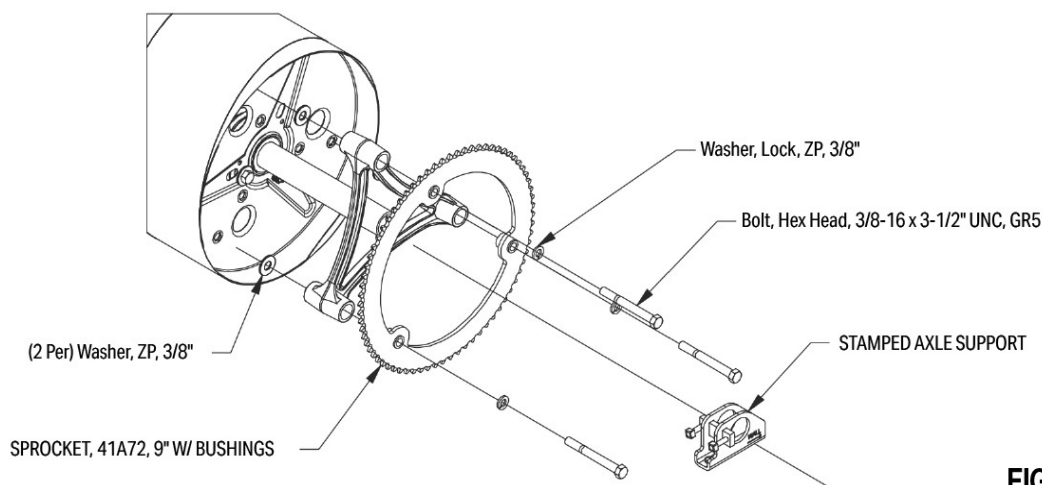
FIGURE 12: ELECTRIC OPERATOR
