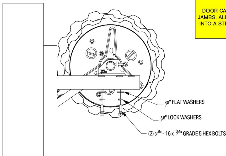
FIGURE 13: SECURING STAMPED AXLE SUPPORT TO BRACKETS
