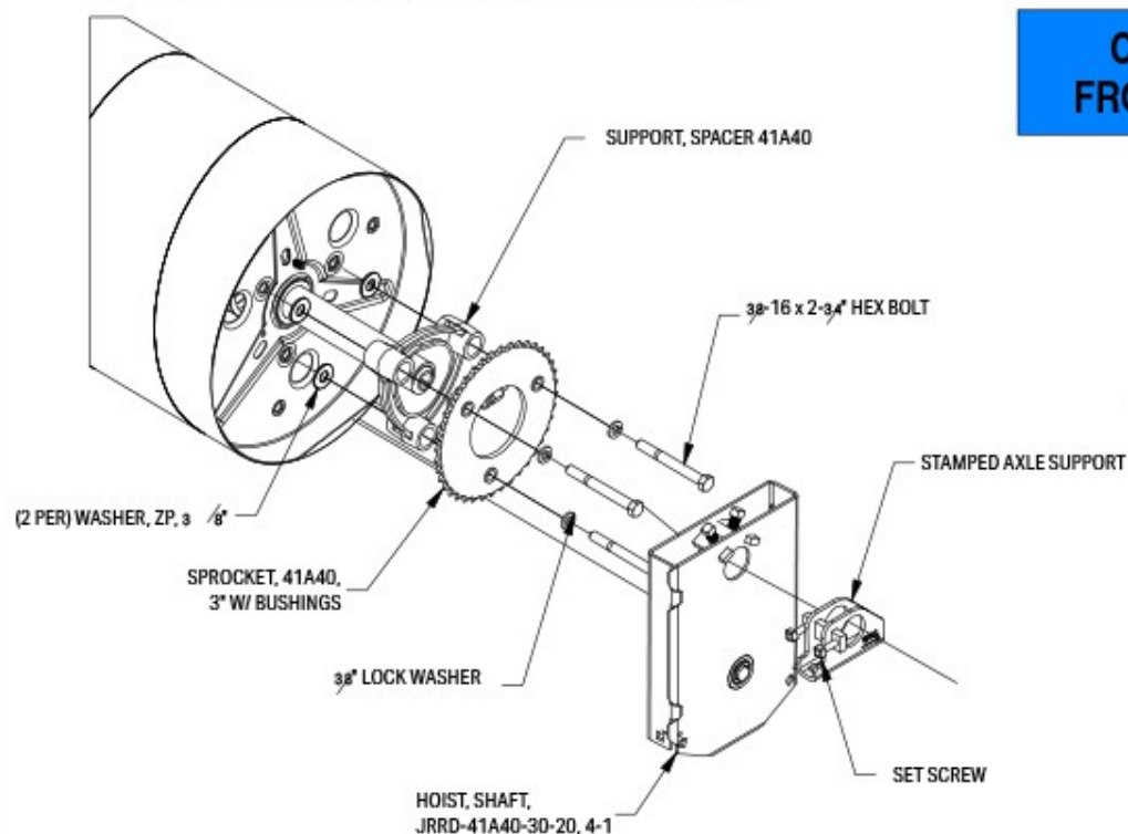
FIGURE 9: CHAIN HOIST 4:1
