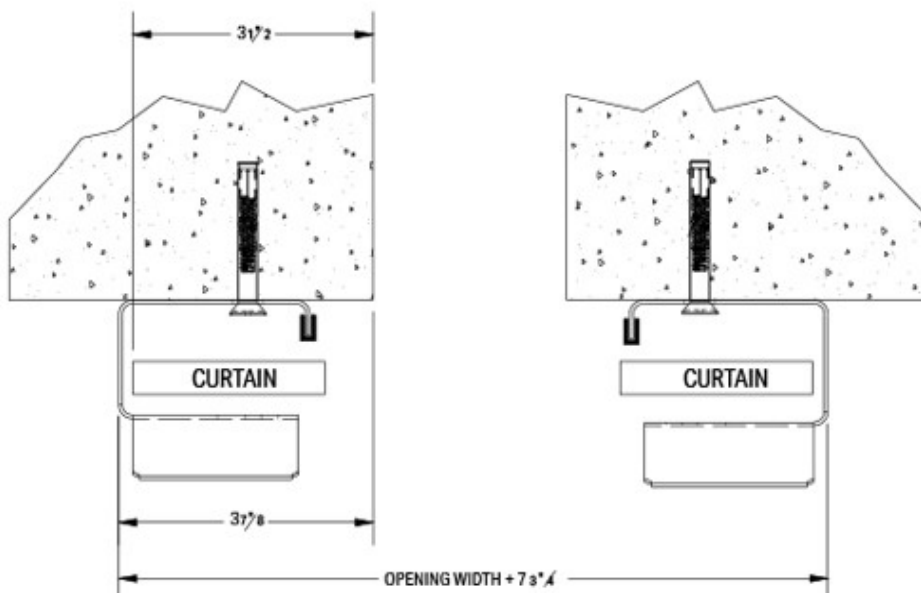
FIGURE 19: CONCRETE / MASONRY JAMBS
