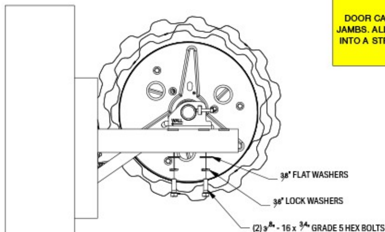
FIGURE 13: SECURING STAMPED AXLE SUPPORT TO BRACKETS
