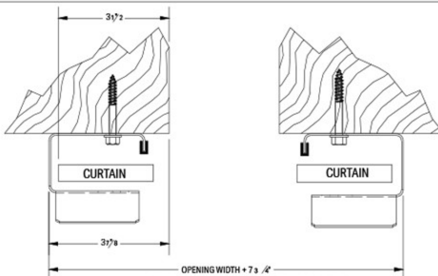
FIGURE 20: WOOD JAMBS
