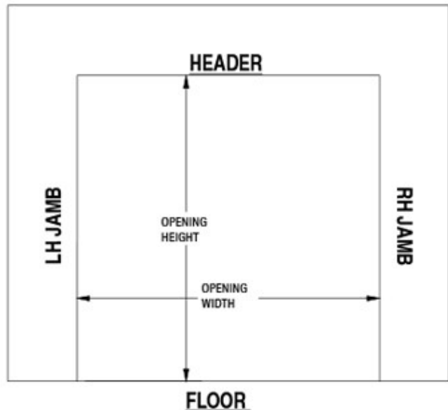
FIGURE 4: WALL OPENING
