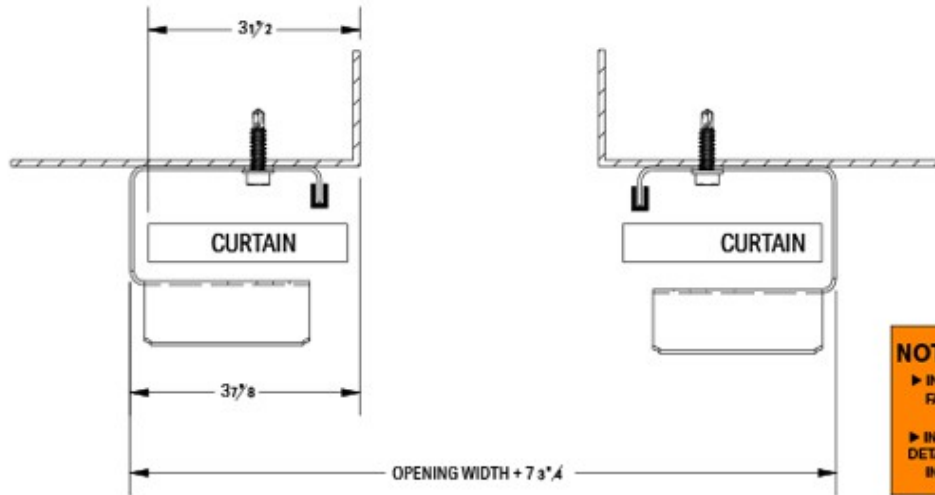
FIGURE 18: STEEL JAMBS
