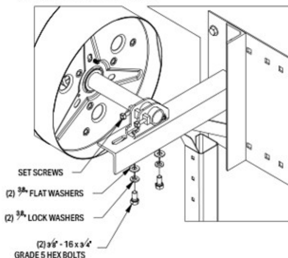
FIGURE 14: SECURING SADDLE
