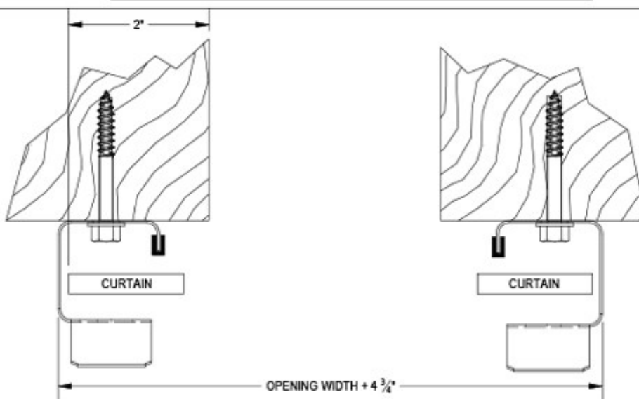
FIGURE 19: WOOD JAMBS
