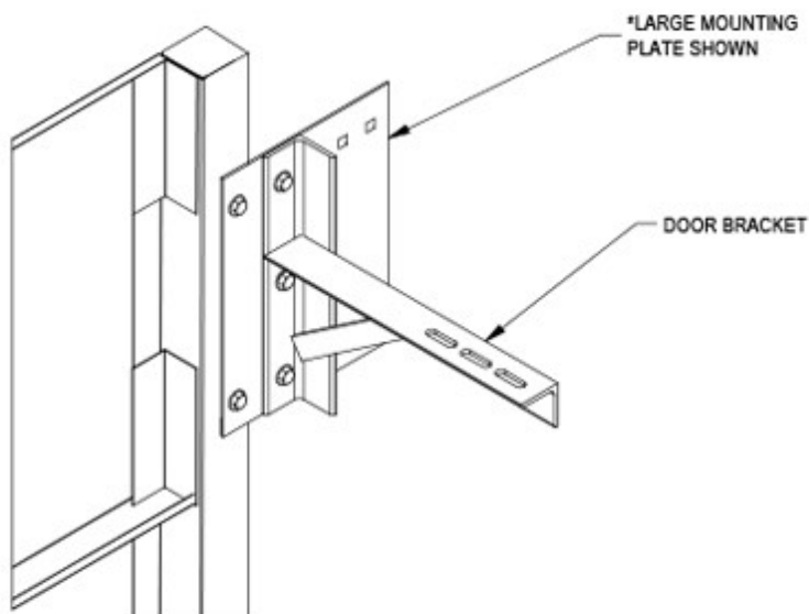
FIGURE 7: DOOR BRACKET TO MOUNTING PLATE
