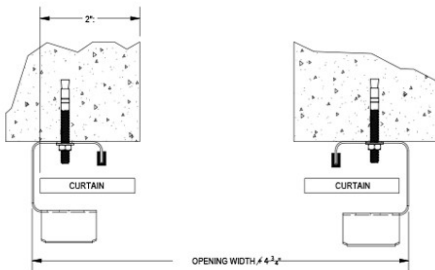
FIGURE 18: CONCRETE / MASONRY JAMBS
