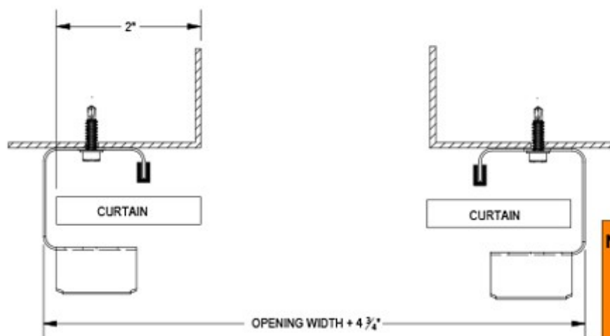
FIGURE 17: STEEL JAMBS
