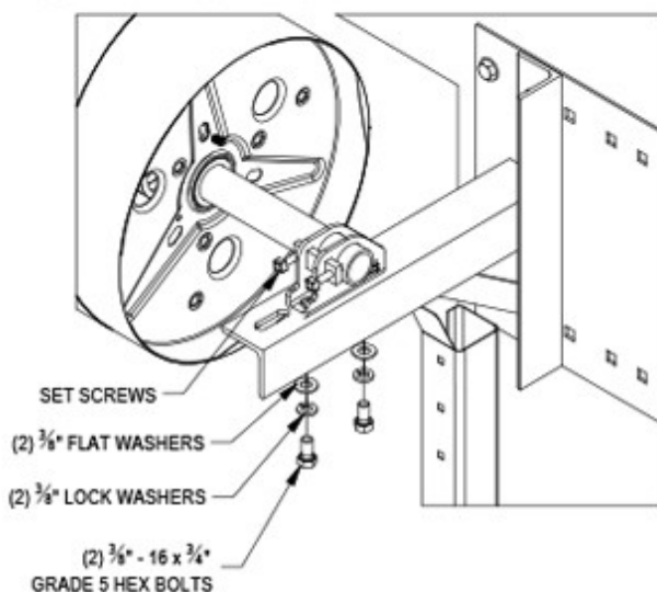
FIGURE 13: SECURING SADDLE
