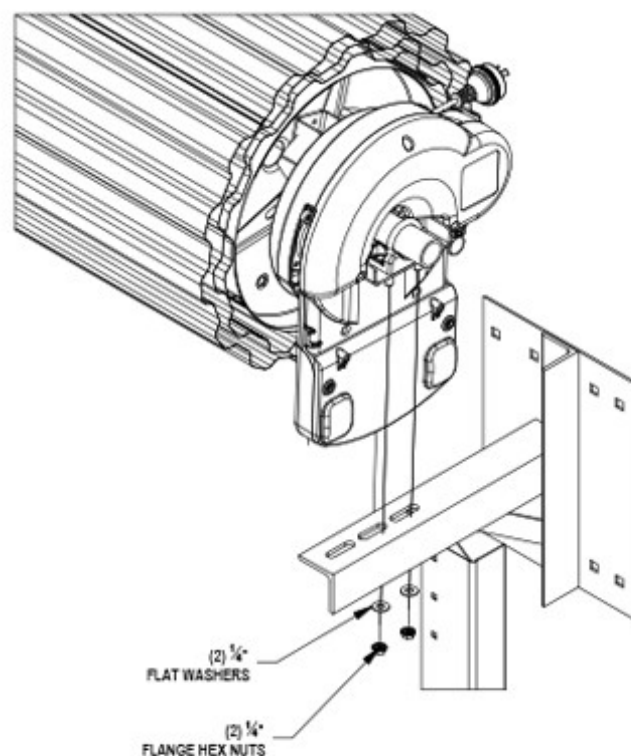
FIGURE 16: ATA OPERATOR END
