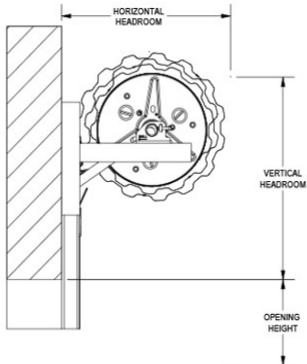
FIGURE 3: SIDEROOM CLEARANCE REQUIREMENT CHART
