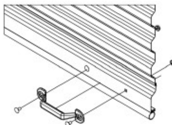
FIGURE 14: HANDLE
