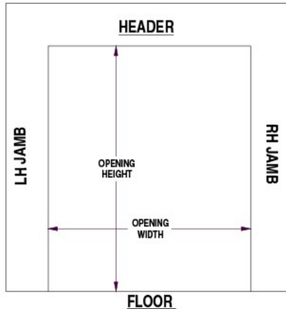
FIGURE 4: WALL OPENING
