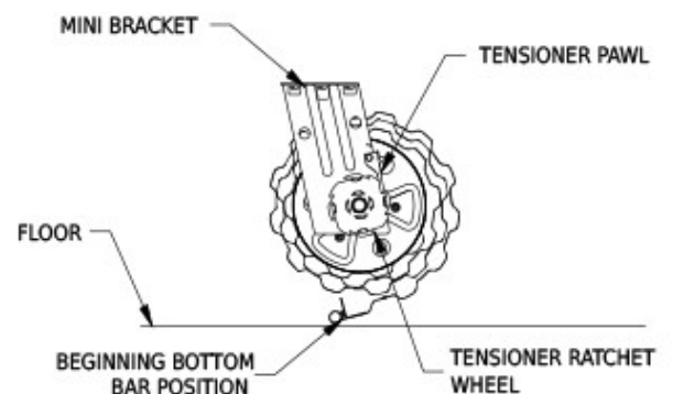
FIGURE 5: POSITION DOOR AND PARTS
